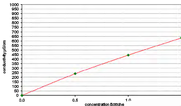
conductivity of BöttcherPro Magnesit in demineralised water
